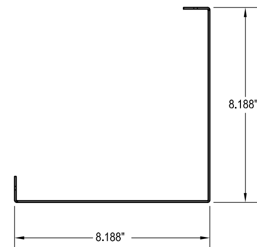
FACE SHEETING SIDE VIEW SCALE 1/4" = 1"
