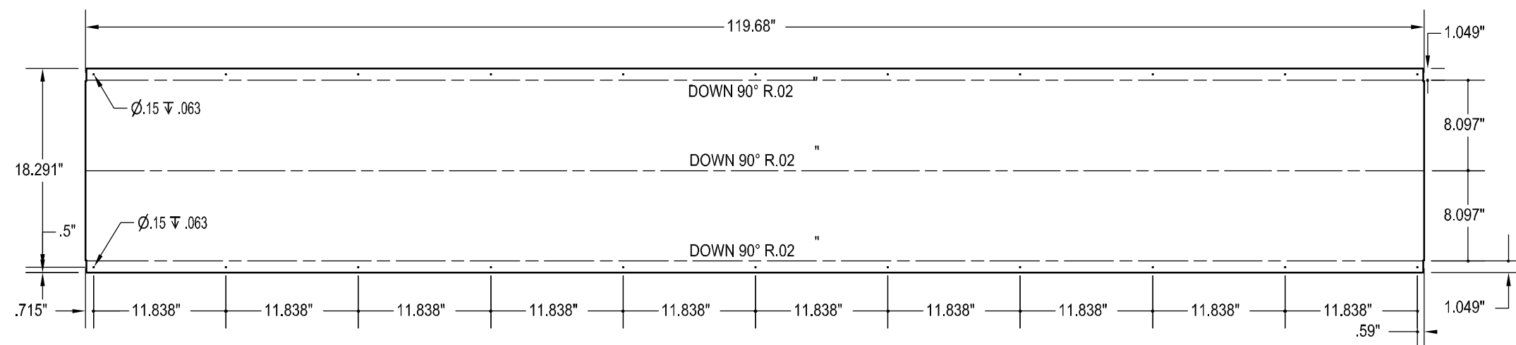
FACE SHEETING FLAT PATTERN SCALE 1" = 1'
